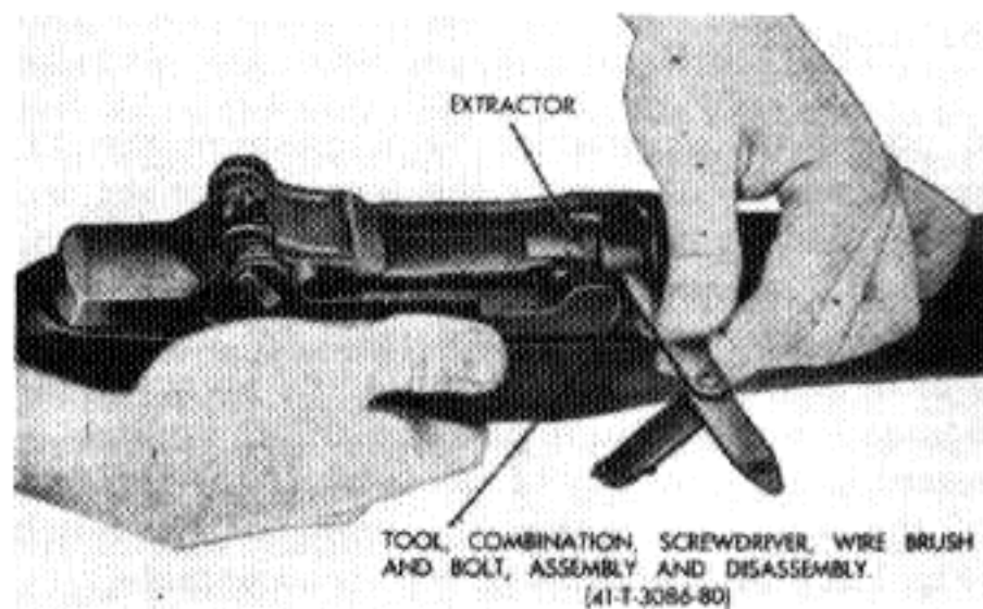
Fig. 116. Removing extractor, bolt in rifle.
