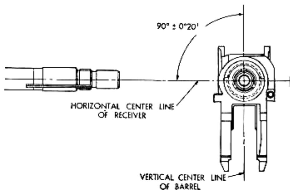
Fig. 140. Barrel and receiver assembly.
