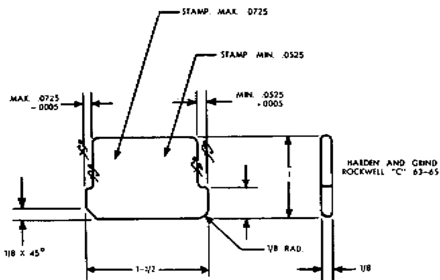
Fig. 109. Height gage.
