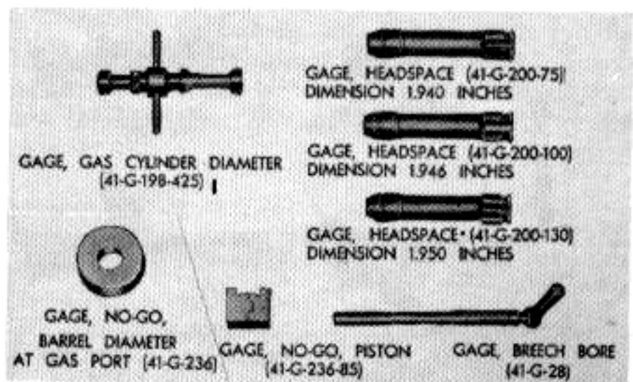
Fig. 98. Gages.
